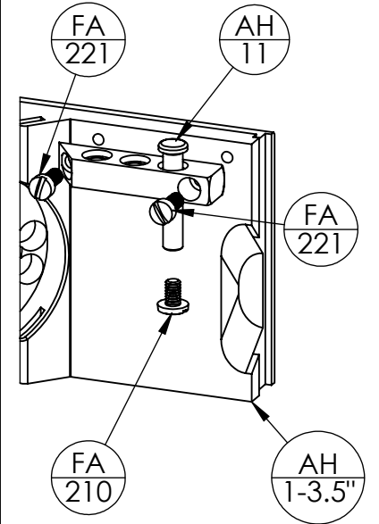
Spring Reduction Option For 3.5" Angle Head
